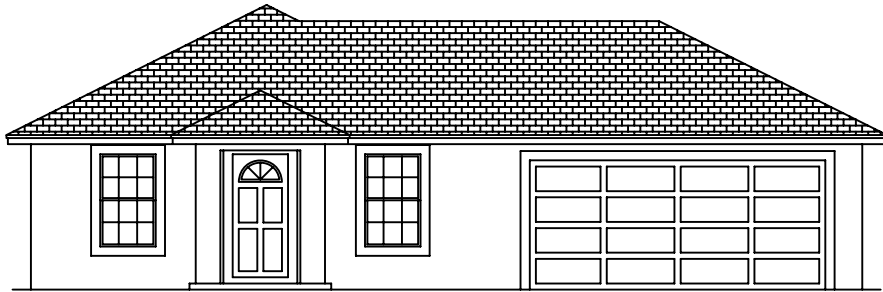
ELEVATION "A"
